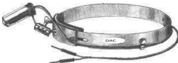
Jansen head light 2052
